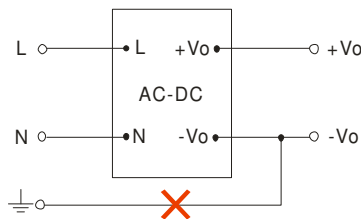
Fig. 2: This application is not supported for this Series.
