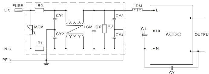
Fig. 3: PPM-SIP-Series Recommended circuit for application require higher EMC standard (external circuit output same as above)
